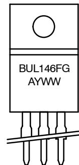
TO-220 FULLPACK CASE 221D STYLE 2 UL RECOGNIZED
